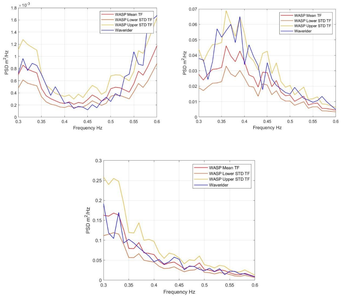
Figure 4.13 – Comparison between Waverider and WASP Spectra for low, medium and high H_s sea-states using Mean Transfer function, with upper and lower standard deviation bounds for, 21 st May 2019 01:30-02:00 (Low H_s ), 13 th May 23:00-23:30 (Med H_s ) and 30 th May 10:30-11:00 (High H_s ) in the frequency range 0.3-0.6 Hertz
