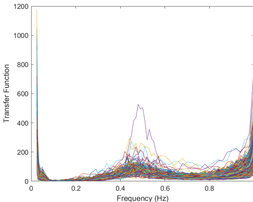
Figure 4.1. Composite graph of monthly transfer functions for March 2019 in the Range 0-1.0 Hertz
