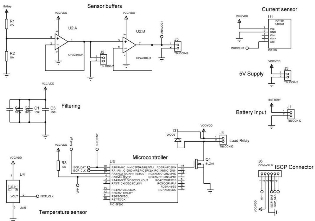
Figure. 3.51. Schematic of the supervisor circuit
