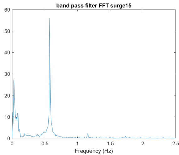
Figure 3.36 – Filtered FFT of the surge from test 15
