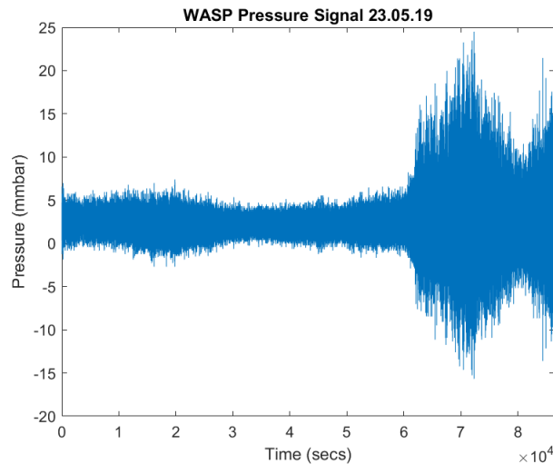
Figure 3.60. 24 hours WASP pressure readings for 23 rd May 2019 - 5-24mmbar, 0.38-01.12m Hs and 2.47-4.39 secs Tz
