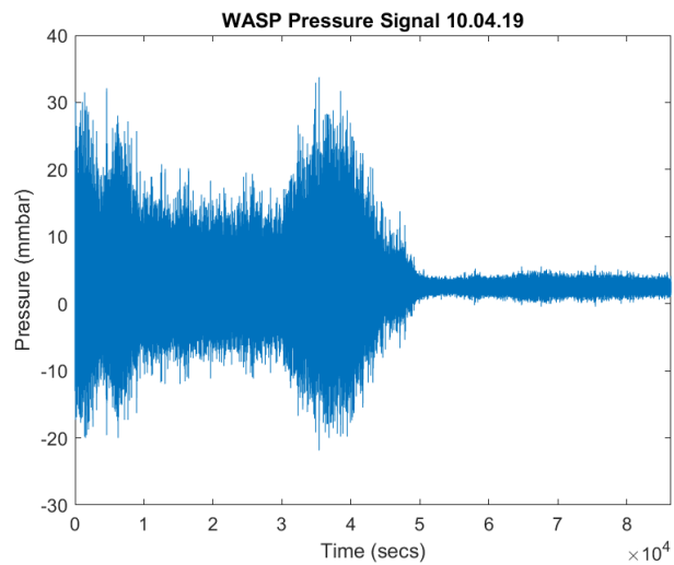
Figure 3.59. 24 hours WASP pressure readings for 10 th April 2019 - 5-32mmbar, 0.27-0.87m Hs and 2.55-6.0 secs Tz
