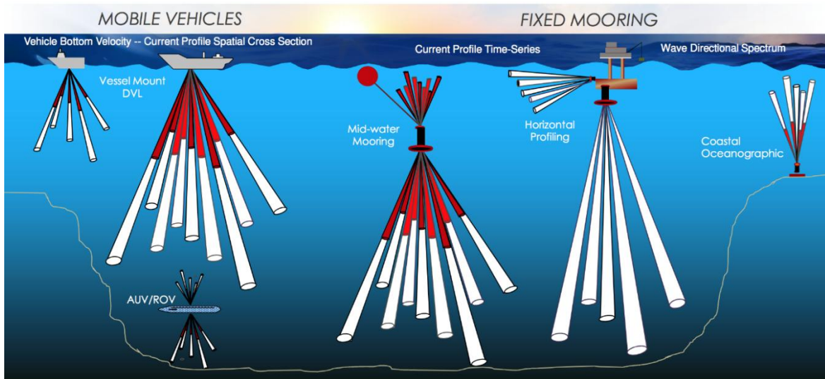
Figure 2.5 – Typical Acoustic Doppler Current Profiler device [164]
