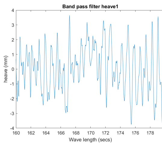
Figure 3.28 – Filtered time series of the heave from test 1 using a band pass filter
