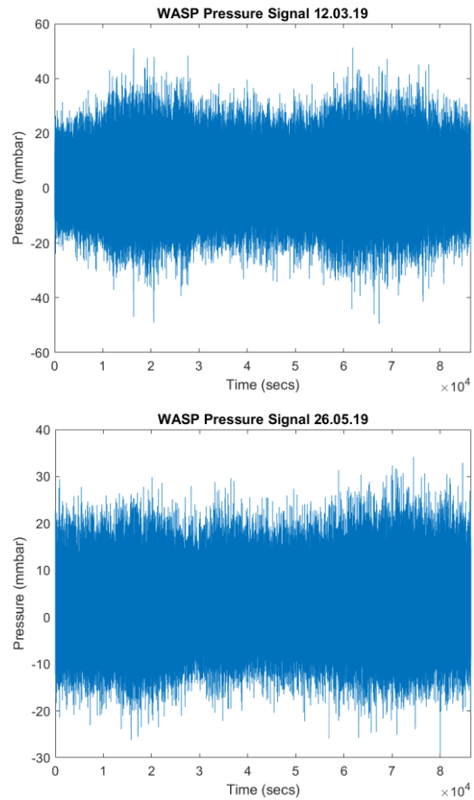
Figure 3.58. 24 hours WASP pressure readings for 12 th March and 26 th May 2019
