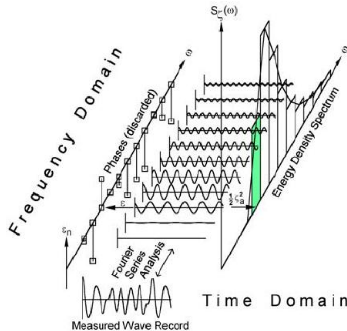
Figure 2.11 – Generating an Energy Density Spectrum [312]
