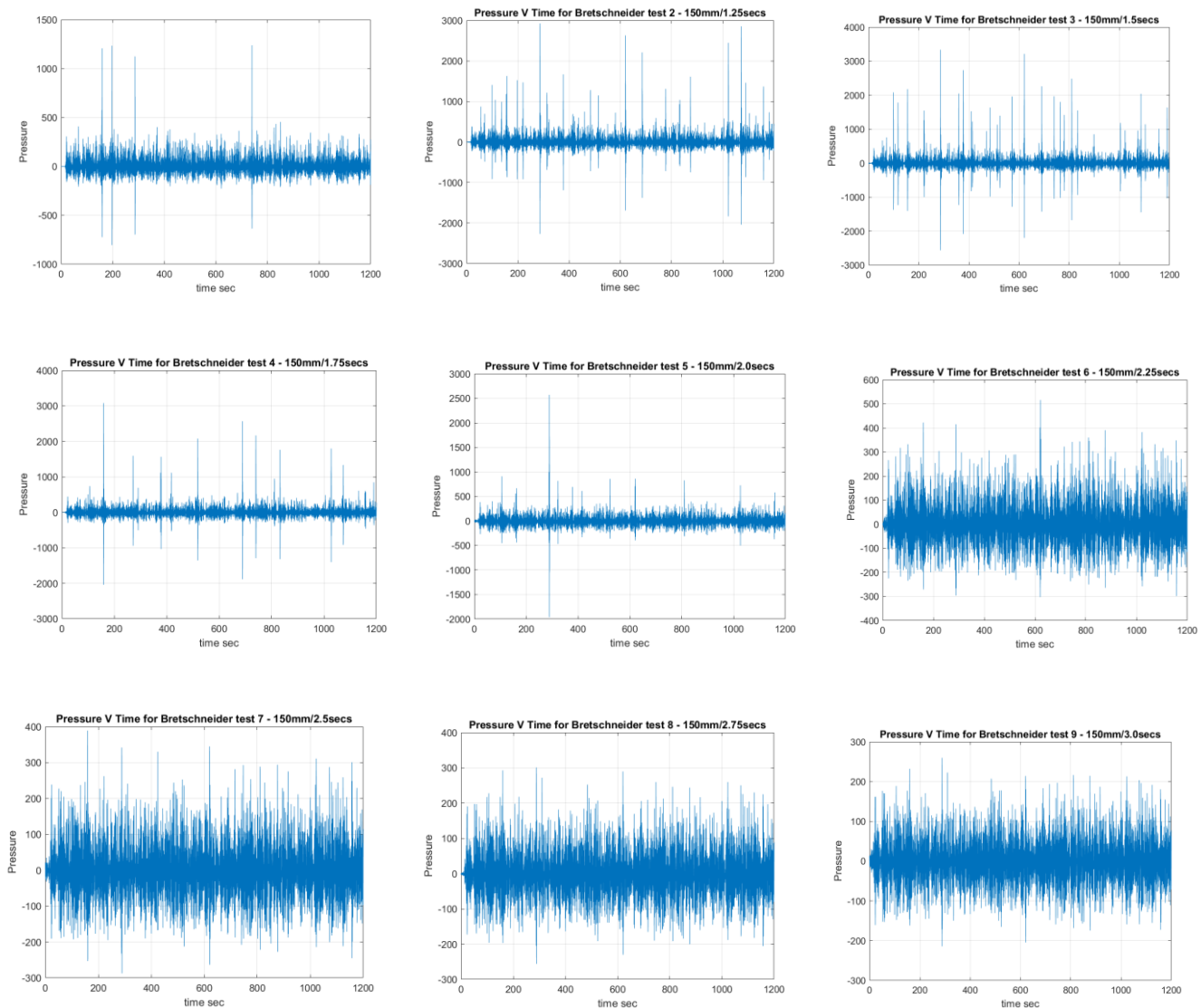
Figure 3.39. Time series of model pressure probe data for tests 1-9 (150mm ranging 1.0-3.0 secs)
