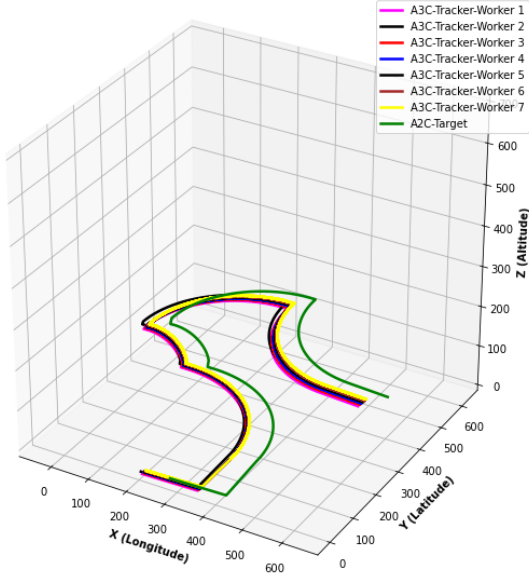
3D Flight Trajectories of A2C Target UAV and A3C Tracker UAVs
