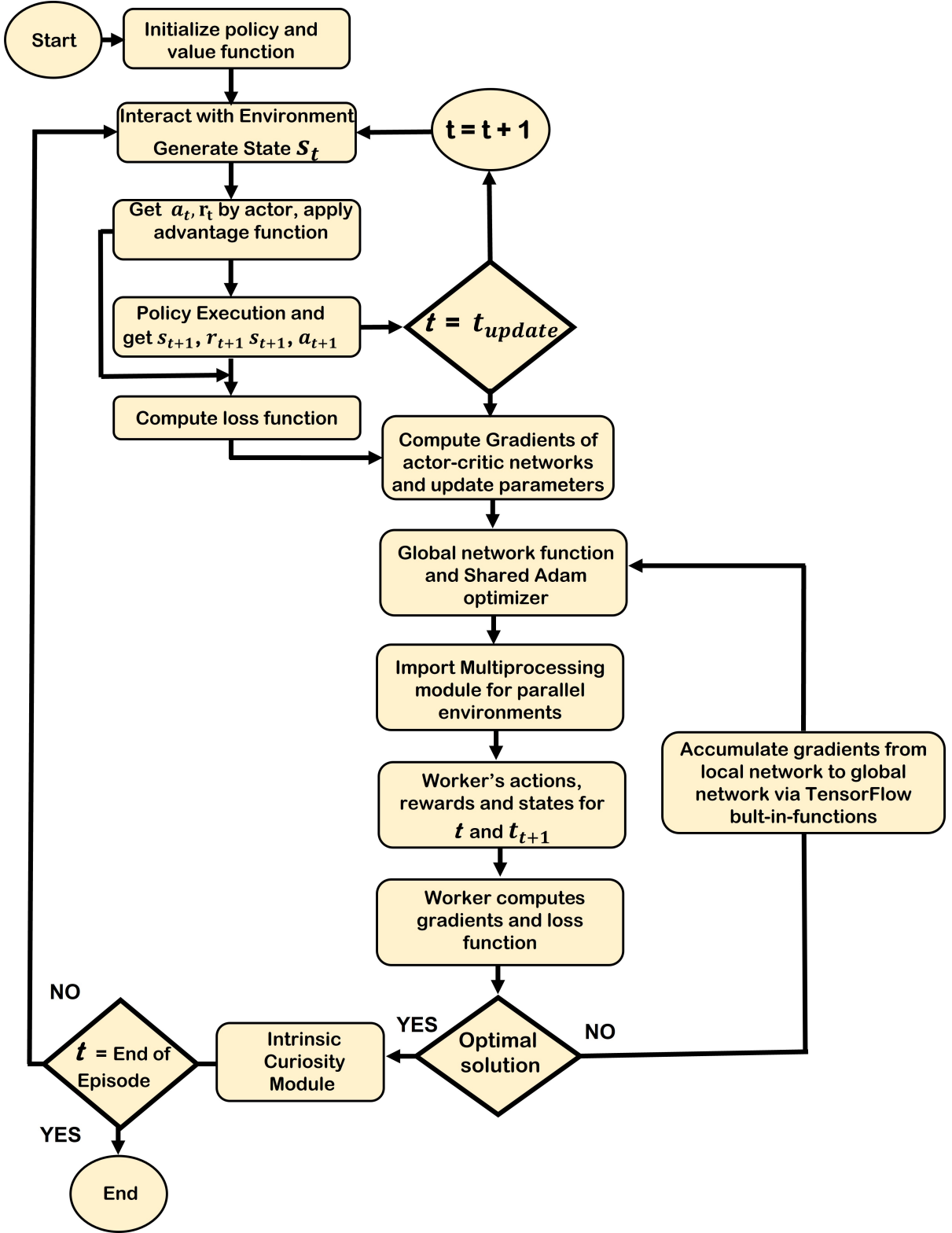
Figure 4.5: Implementation of A3C algorithm.
