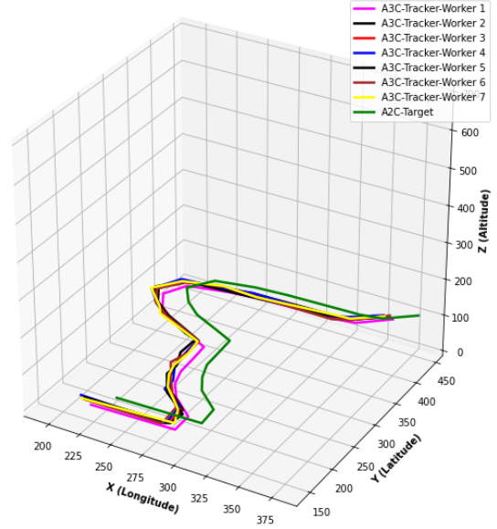
3D Flight Trajectories of A2C Target UAV and A3C Tracker UAVs
