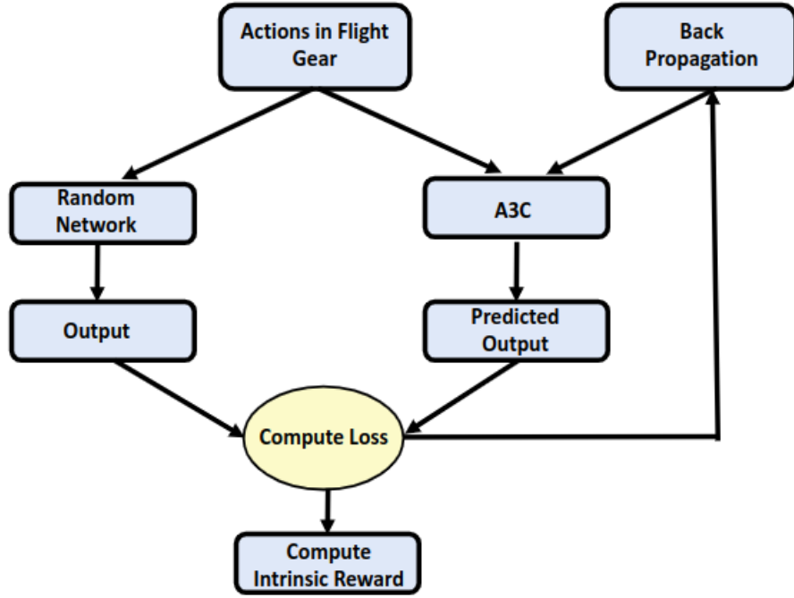
Figure 4.6: Implementation of ICM.
