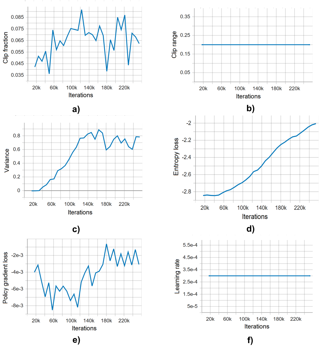
Figure 5.6: Graphical results of PPO algorithm a) Clip fraction b) Clip range c) Variance d) Entropy loss e) Policy gradient loss f) Learning rate.
