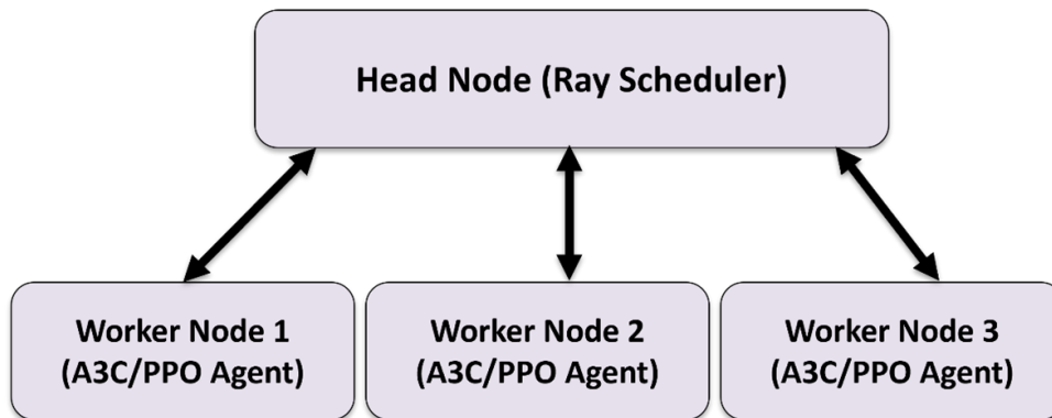
Figure 4.10: Flowchart shows Ray handles the communication between the separate Nodes
