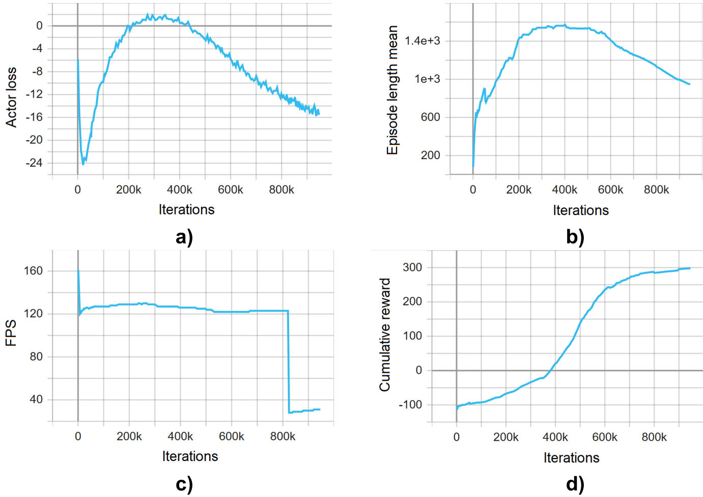
Figure 5.2: Graphical results for the implementation of A3C algorithm a) Actor loss, b) Episode length mean, c) FPS, d) Cumulative reward.
