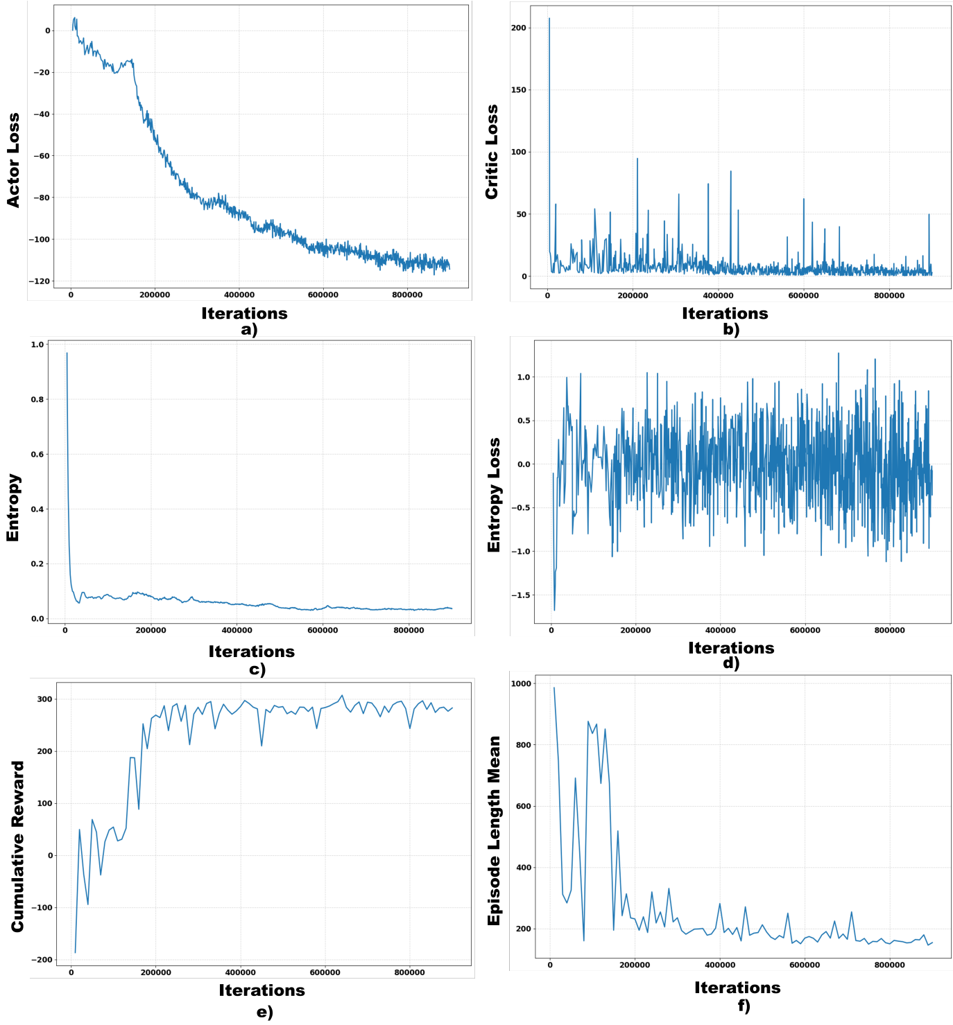
Figure 5.1: Graphical results to show the implementation of A2C algorithm a) Actor loss b) Critic loss c) Entropy d) Entropy loss e) Cumulative reward f) Episode length mean
