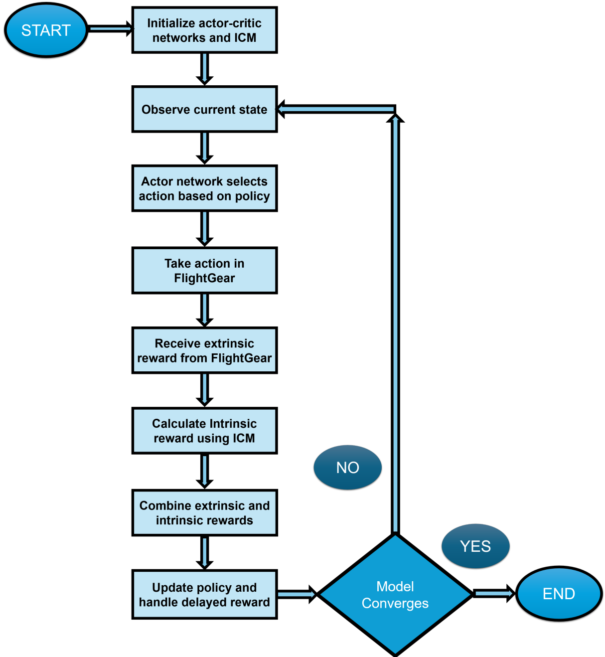
Figure 4.7: Framework to overcome the problem of delayed reward using A3C-ICM model.
