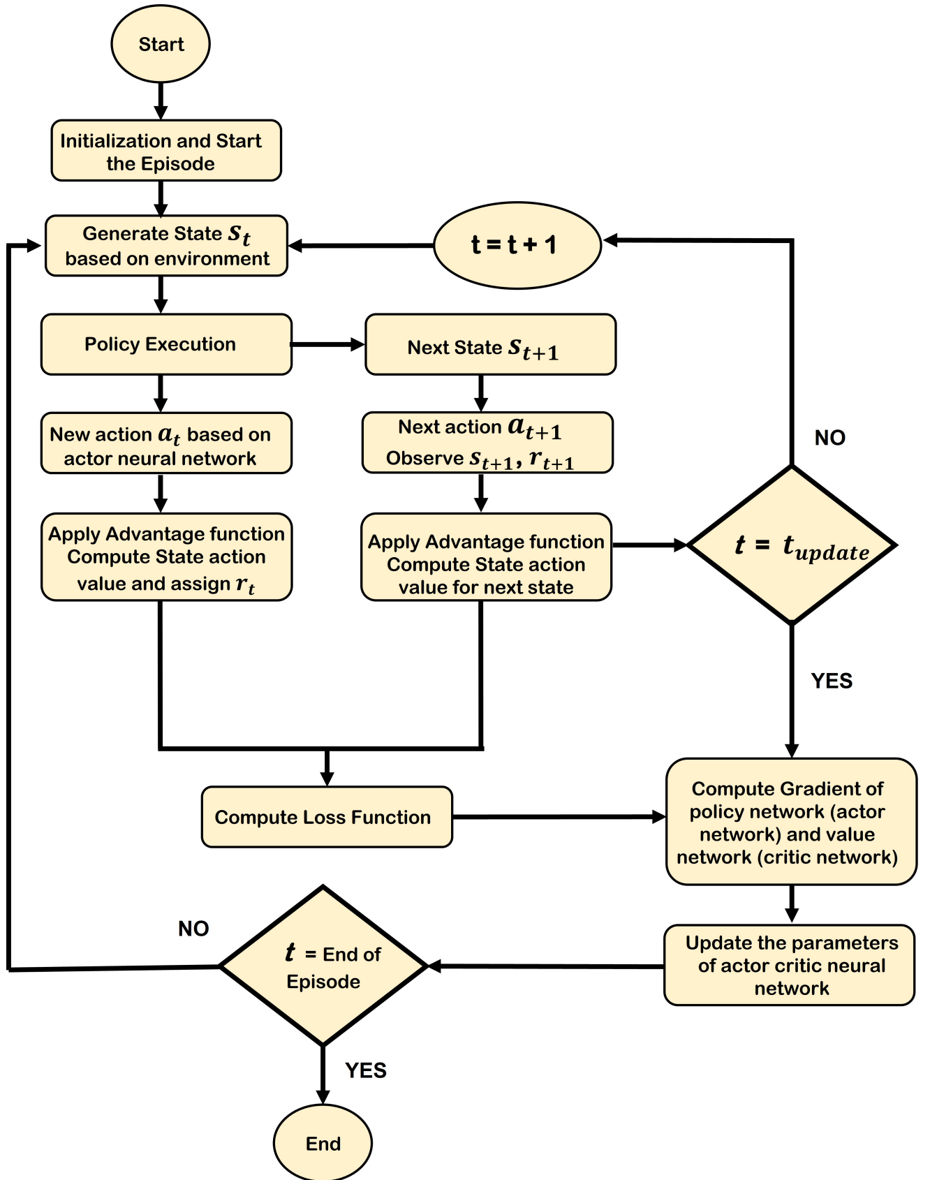
Figure 4.4: Implementation of A2C algorithm
