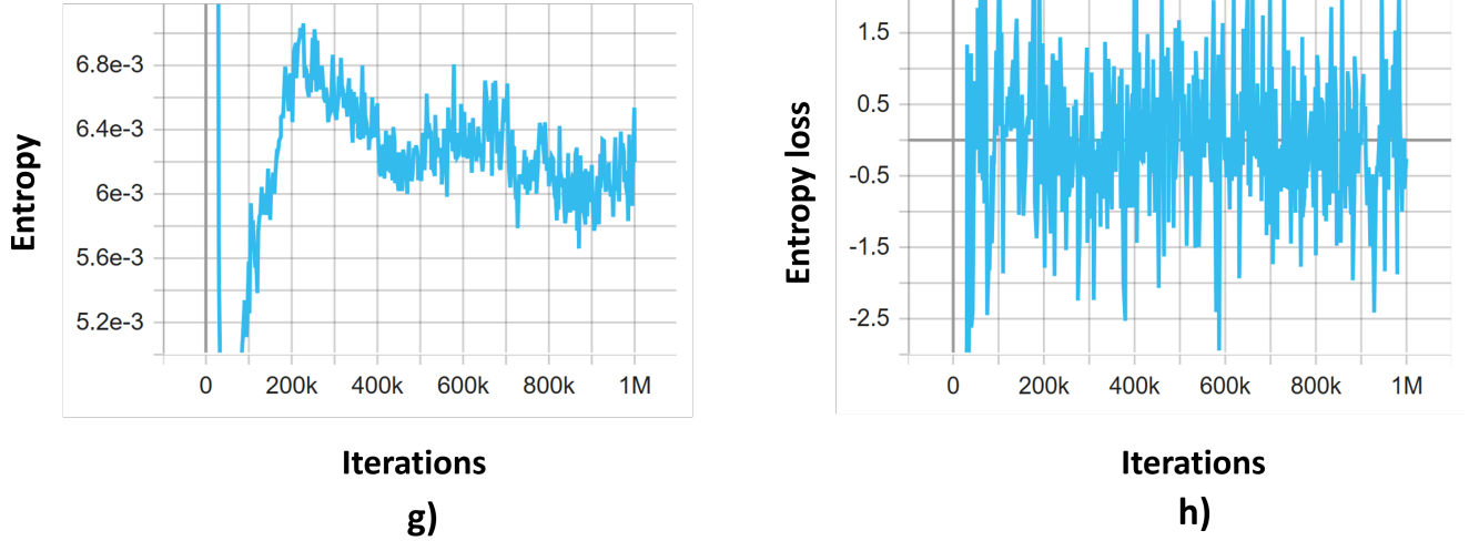
Figure 5.5: Graphical illustration of A3C performance g) Entropy h) Entropy loss.
