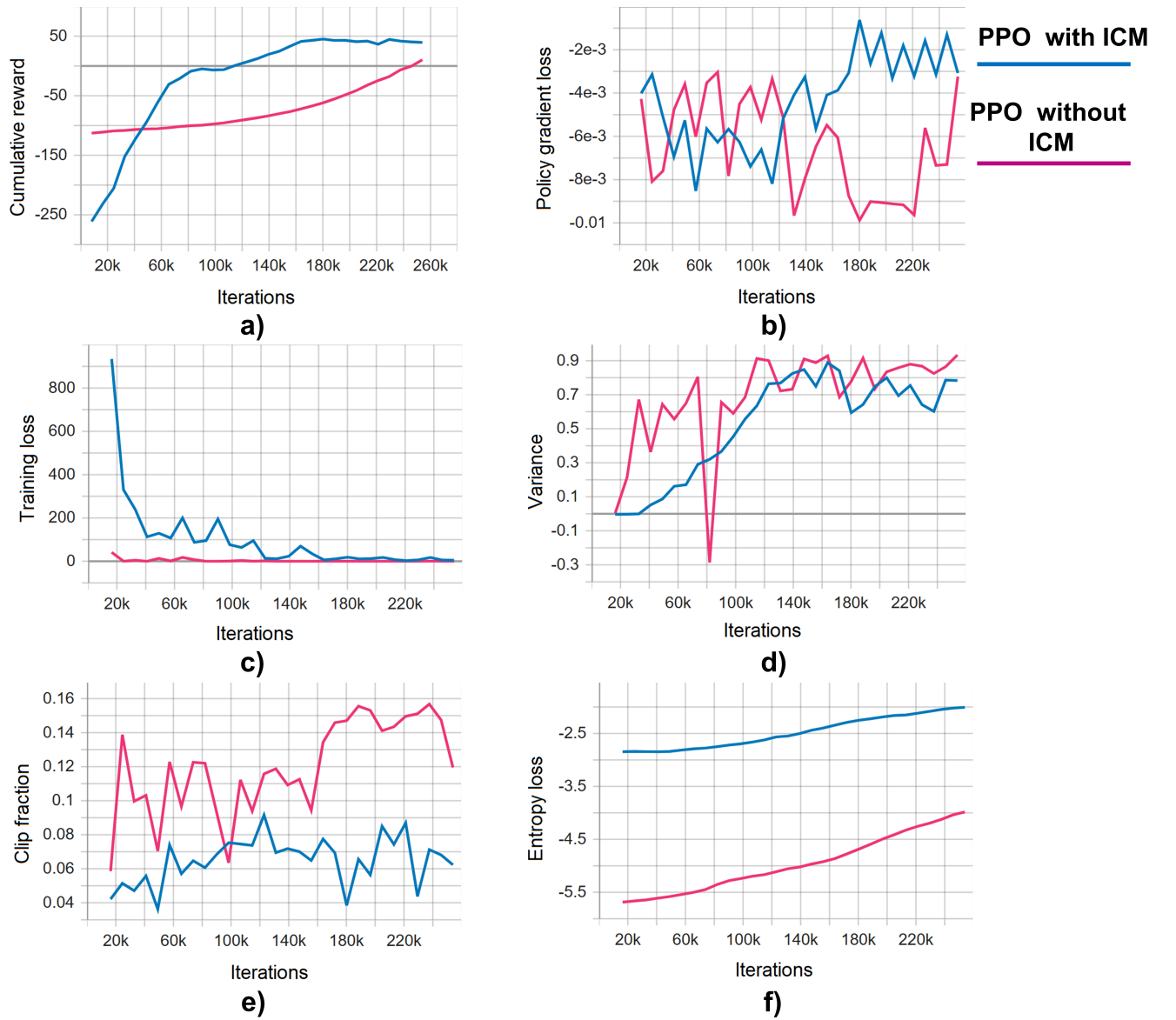
Figure 5.9: Graphical results to show the comparison of performance between PPO with ICM and PPO without ICM a) Cumulative reward b) Policy gradient loss c) Training loss d) Variance e) Clip fraction f) Entropy loss.
