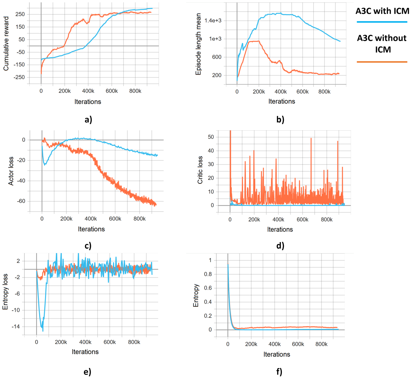
Figure 5.8: Graphical results to show the comparison of performance between A3C with ICM and A3C without ICM a) Cumulative reward b) Episode length mean c) Actor loss d) Critic loss e) Entropy loss f) Entropy.
