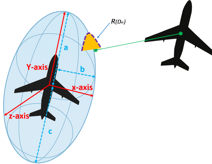
Figure 4.9: Illustration of the calculation of reward by placing the Gaussian reward function on the boundary of an ellipsoid. The UAV inside the ellipsoid corresponds to a tracking UAV under consideration that has to compute its reward. The other UAV is either a target or some other tracker.
