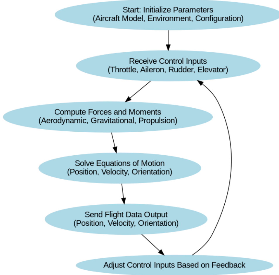
Figure 4.2: Flowchart illustrating the working mechanism of JSBSim.
