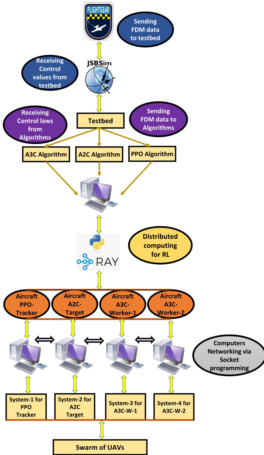
Figure 4.11: Distributed learning computing framework of Testbed for swarm of UAVs.
