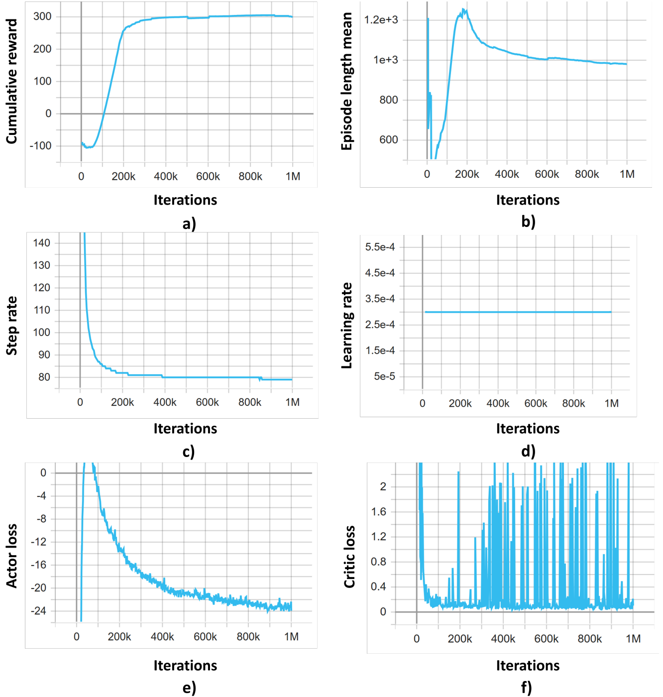
Figure 5.4: Graphical illustration of A3C performance for seven workers a) Cumulative reward b) Episode length mean c) Step rate d) Learning rate e) Actor loss f) Critic loss.
